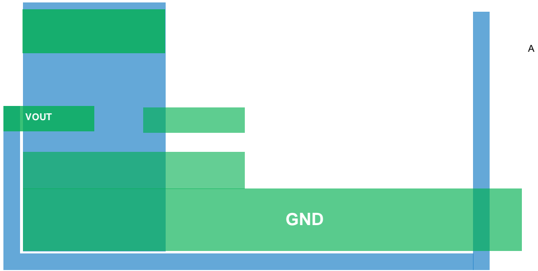
Figure 22. PCB Layout Example (SCT2120 TTBR)
